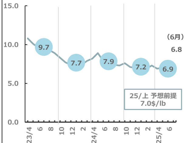
Ni($/lb)
